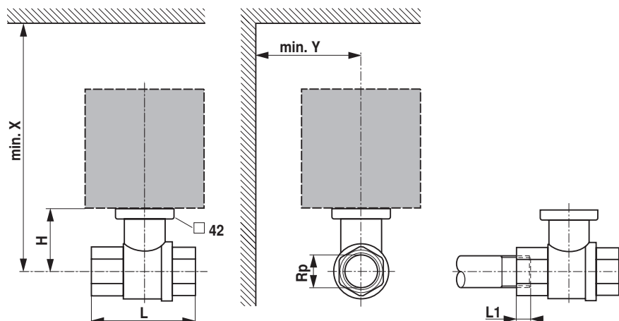
Dimensional drawings
